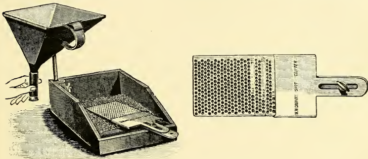
W. W. Greener's Shot-Counting Apparatus.
